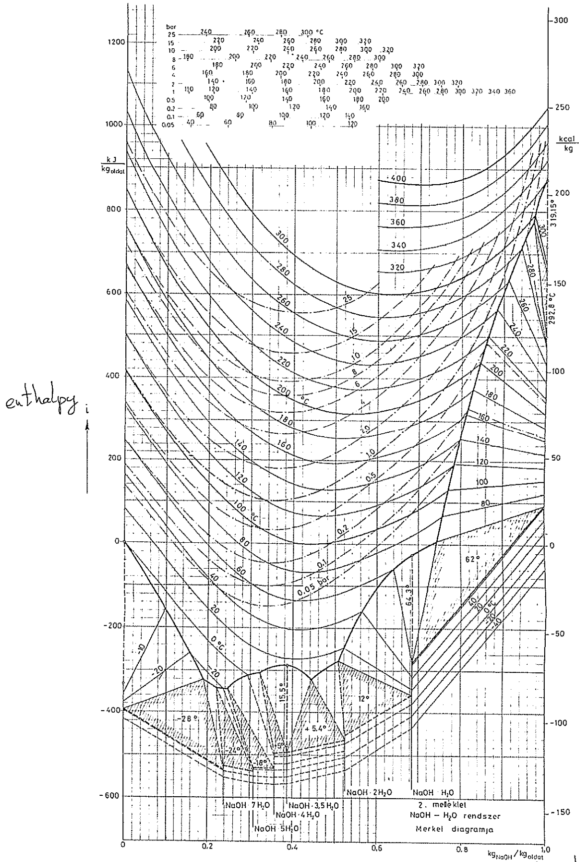
Merkel-plot of system NaOH - H 2 O
